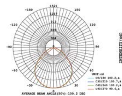
LUMINOUS INTENSITY DISTRIBUTION
